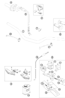
HANDLEBAR, CONTROLS
